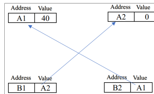
Figure 3: Status of the pointers after swapping
