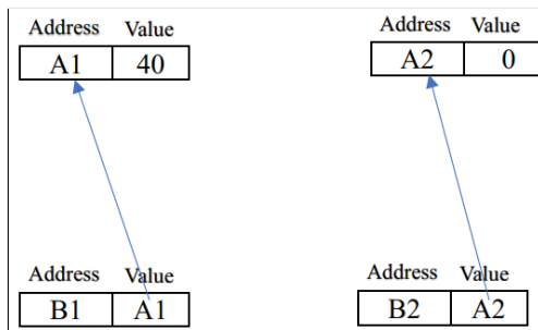
Figure 2: Status of the pointers before swapping
